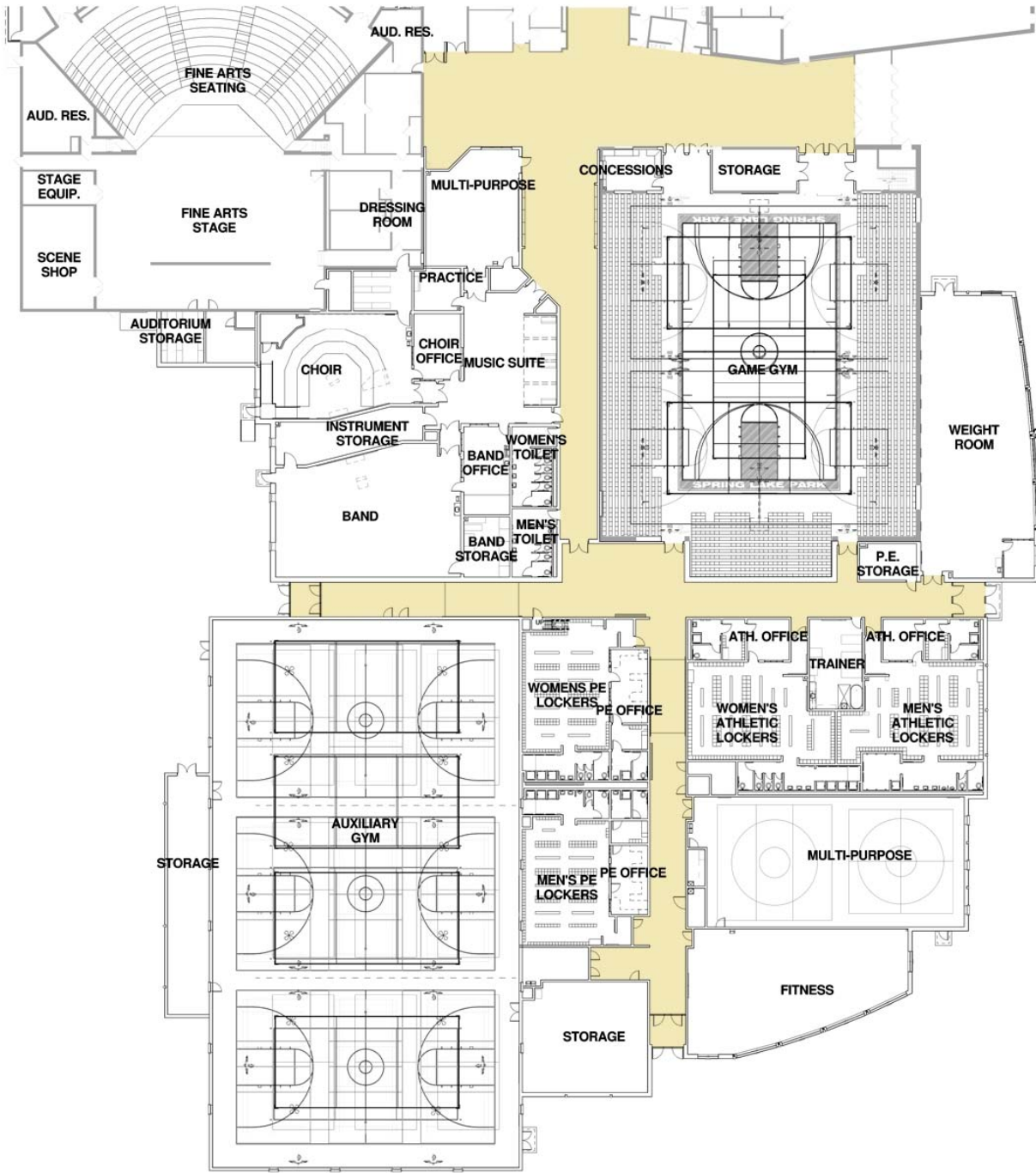
PHASE 1 - MAIN FLOOR PLAN 1/16" = 1'-0"
